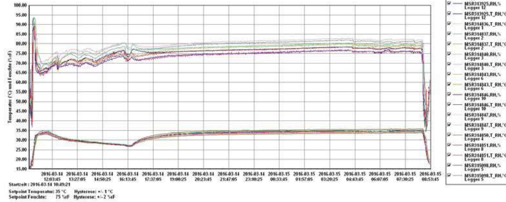
Temperature and Relative Humidity Data. Equipment Commissioning QUADRIX® System KC 300-150 #872, 14./15.03.2016
