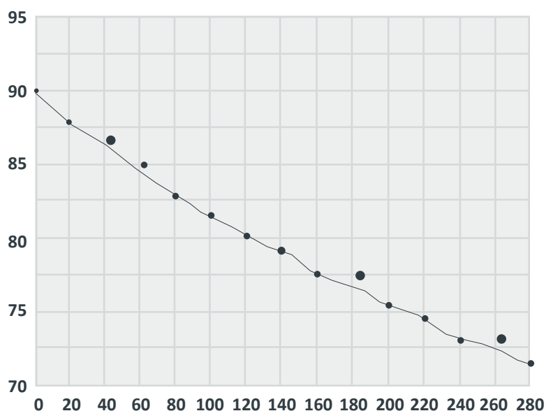
% Excess Air in Steam-Flue Gas Mixture
